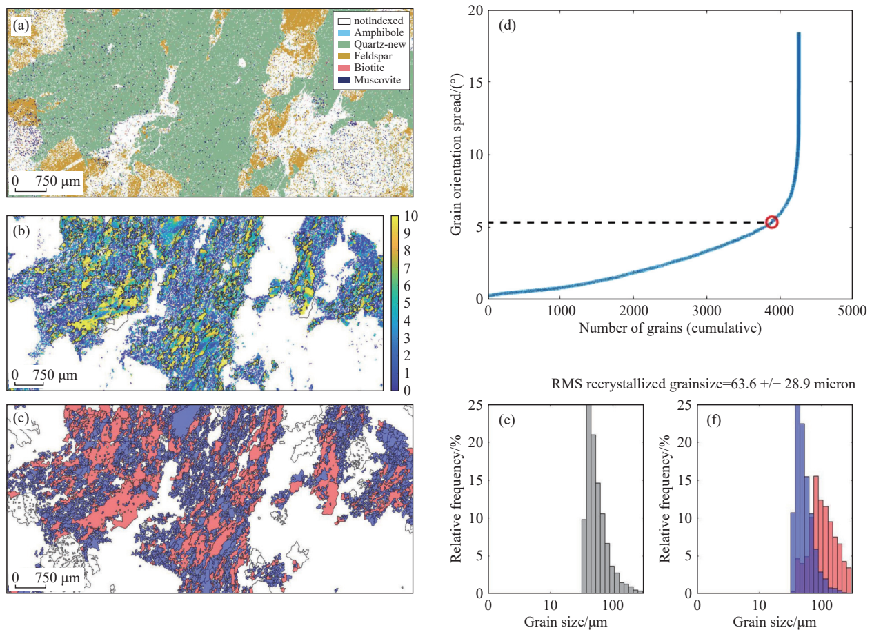
Fig. 7. Recrystallized quartz grain size data and associated microstructures for representative mylonites. (a) Phase diagram of sample 19TL07 minerals from EBSD analysis; (b) Orientation distribution (GOS) of each grain; (c) Distribution of recrystallized particles (blue) and residual particles (red) separated by GOS; (d) Cumulative plot of sample 19TL07 particle count vs. particle orientation distribution; (e) Grain size distribution histogram of all particles for sample 19TL07; (f) Grain size distribution histogram of residual and recrystallized grain of sample 19TL07.
