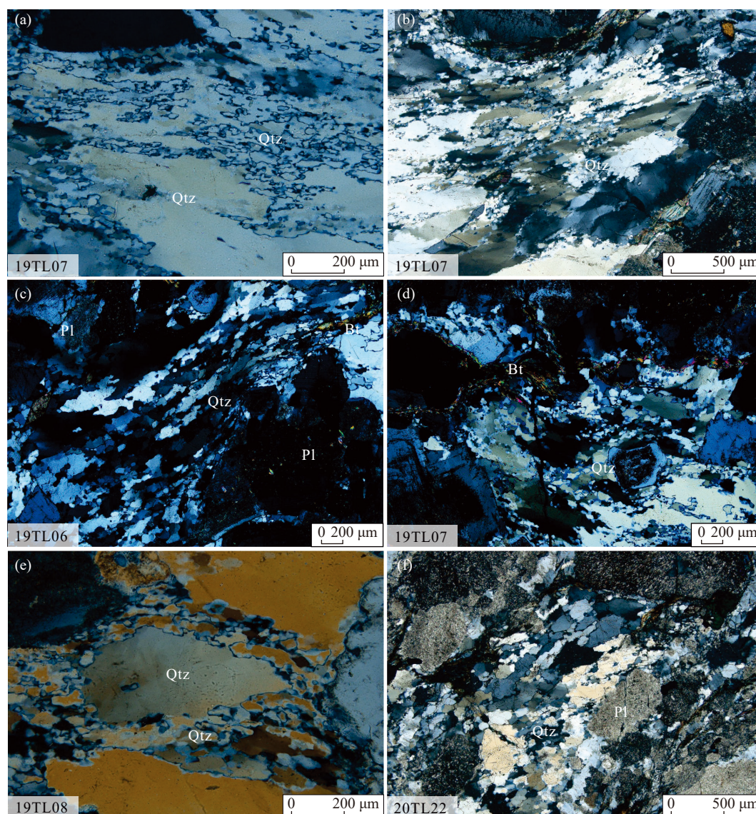
Fig. 5. Photomicrographs showing recrystallization of quartzes in mylonites. (a) Sub-particle rotational recrystallization; (b) expansion type recrystallization; (c) particle boundary migration rejunction crystal; (d) subparticle rotational recrystallization; (e) Nuclear mantle structure composed of subparticle rotational recrystallization; (f) Particle boundary migration recrystallization.
