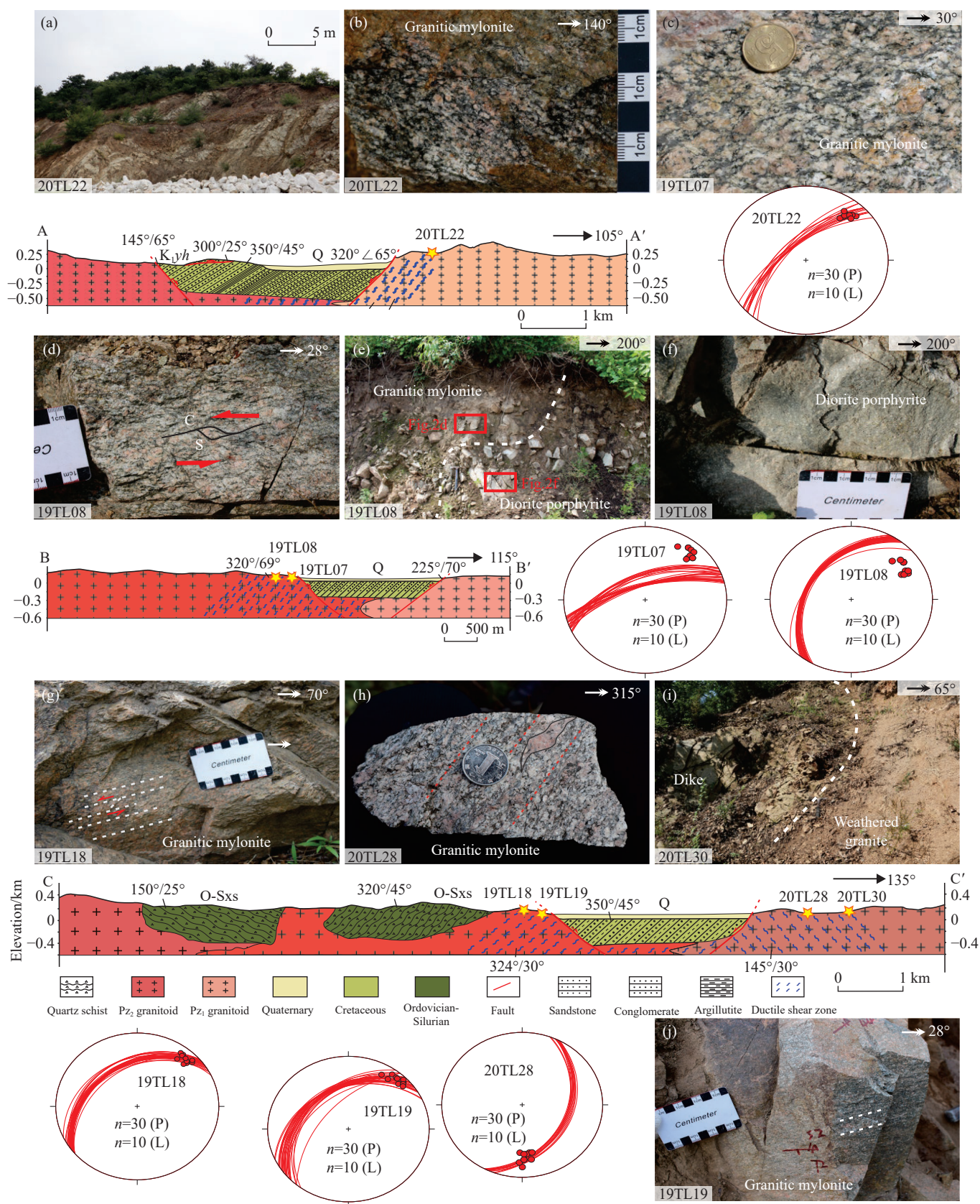
Fig. 2. Transects, field photographs, and projections of structural elements through the Weiyuanpu-Yehe shear zone. (a) Fault zone dominated by shear bends, breccia, and gouge (stop 20TL22); (b) Granitic protomylonite (stop 20TL22); (c) Outcrops of granitic mylonite of the ductile shear zone on the west side (stop 19TL07); (d) S-C fabrics that were defined by feldspar and elongated quartz and hornblende and biotite, indicating a sinistral strike-slip (19TL08); (e) Undeformed porphyrite dike intruded into the granitic mylonite in the western side of shear zone (stop 19TL08); (f) Undeformed diorite porphyrite dikes (stop 19TL08); (g) S-C fabrics in protomylonite (stop 19TL18); (h) Potassium feldspar asymmetry porphyroclasts in protomylonite (stop 20TL28); (i) dike intruded into the granite within the shear zone near the Weiyuanpu town (stop 20TL30); (j) Granitic mylonite defined by mineral lineation (stop 19TL19).
