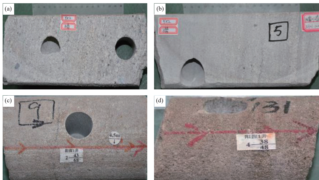
Fig. 2. Core samples from Yangxia Formation and Ahe Formation in Yangxia sag. a–Well YX-2, 5290.3 m, J_{1Y} , gravelly coarse sandstone; b–Well YX-2, 5301.1 m, J_{1Y} , coarse-medium sandstone with positive grain sequence; c–Well YT-1, 7712.2 m, J_{1a} , grey thick medium sandstone; d–Well YT-1, 7798.4 m, J_{1a} , gray sand-bearing coarse grained rock.
