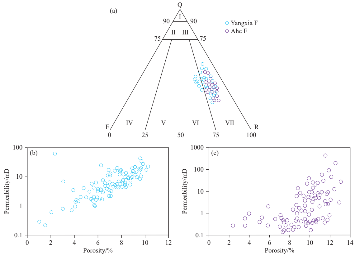
Fig. 7. Rock classification of sandstone reservoirs of Yangxia and Ahe Formations in Yangxia sag (a) and their porosity and permeability comparison (b and c). I—Quartz sandstone; II—feldspar quartz sandstone; III—lithic quartz sandstone; IV—feldspar sandstone; V—lithic feldspar sandstone; VI—feldspar lithic sandstone; VII—lithic sandstone.
