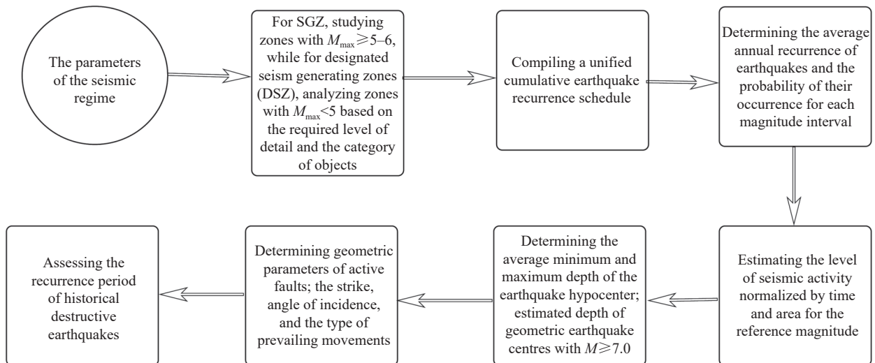
Fig. 5. Process of setting the parameters of the seismic regime (after Silacheva NV et al., 2018).
