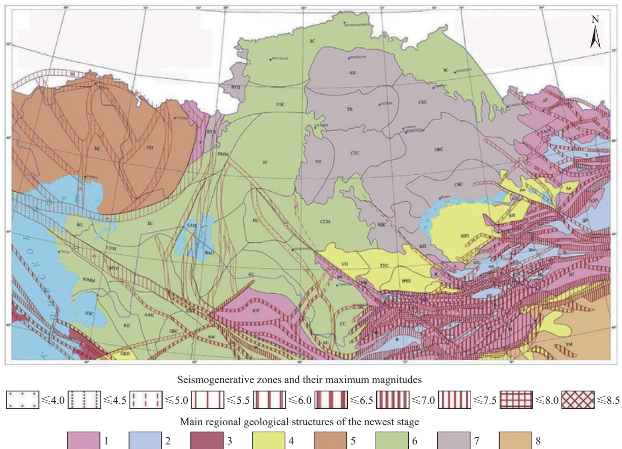
Fig. 1. Map of seismogenerative zones of the Kazakhstan's Earth crust (after Silacheva NV et al., 2018). 1–epiplatform orogens; 2–interand intra-montane depressions; 3–epigeosynclinal orogens; 4–orogen and platform conjunction zones; 5–ancient platform with Paleozoic Cenozoic slab complex (the Caspian basin); 6–young Turan epihercine platform with MesozoicCenozoic slab complex; 7–Kazakh Shield (consolidated basement) of the young platform; 8–Tarim Massif.
