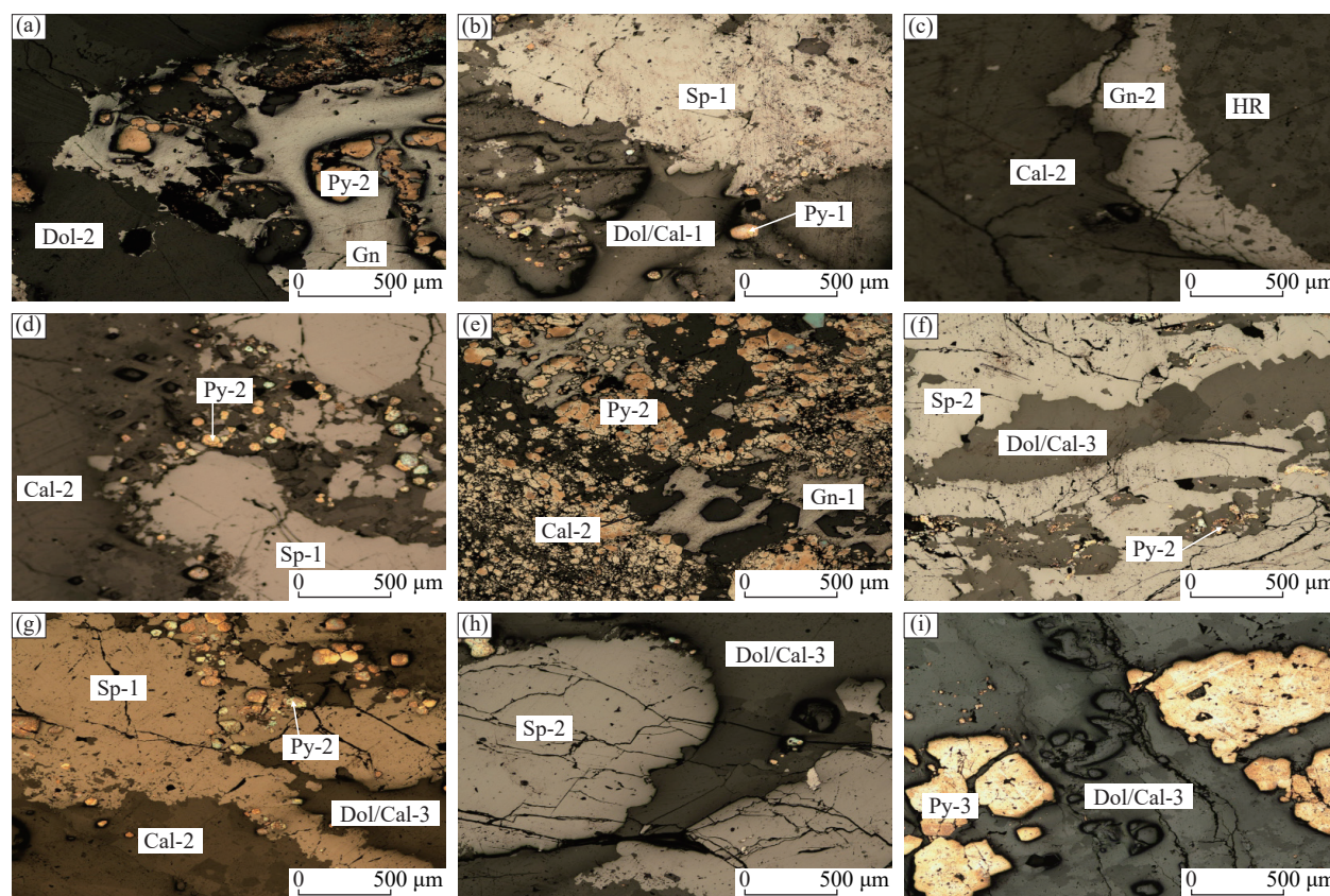
Fig. 7. Textural and structural features of minerals in the Maoping deposit under a microscope. (a) Gn-1 replaces Py-2, and both coexists with Dol-2; (b) Hypidiomorphic-xenomorphic Py-1 coexists Dol/Cal-1 veinlets in the HR, but both interspersed by Sp-1; (c) Cal-2 coexists with banded Gn-2; (d) Cal-2 coexists with Sp-1, and replaces granular Py-2; (e) Cal-2 coexists with Gn-1, and both replace fragmentary Py-2; (f-h) Sp-2 coexists with granular Py-2 and Cal-2, but interspersed by Dol/Cal-3 veinlets; (i) Py-3 replaced by Dol/Cal-3 veinlets.
