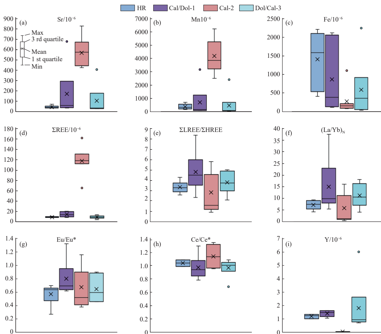
Fig. 10. Box plots of (a) Sr, (b) Mn, (c) Fe, (d) \Sigma REE, (e) \Sigma LREE/ \Sigma HREE, (f) (\text{La/Yb})_N , (g) \text{Eu/Eu}^* , (h) \text{Ce/Ce}^* , and (i) Y values of hydrothermal calcites from the Maoping Pb-Zn deposit.
