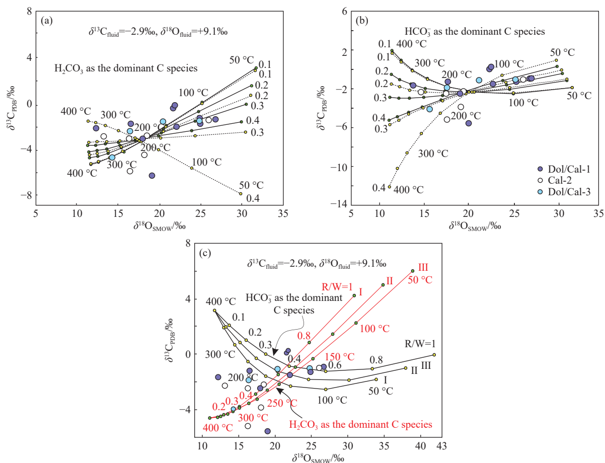
Fig. 15. (a) H 2 CO 3 and (b) HCO 3 - as the dominant carbon species in simulation diagram of CO 2 degassing for the hydrothermal carbonate minerals; (c) simulation diagram of water-rock interaction for hydrothermal carbonate minerals.
